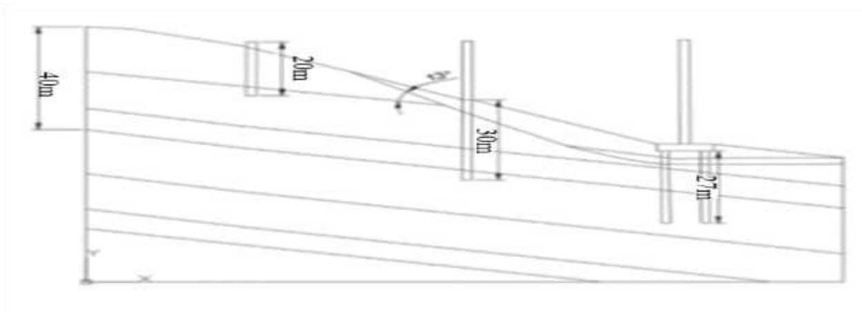
Figure 1: Calculation model of Zhangyoufang Bridge
