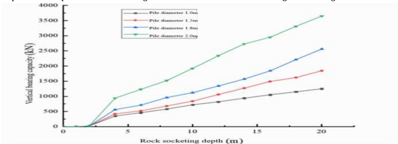
Figure 5: Distribution of vertical bearing capacity of different pile diameters
