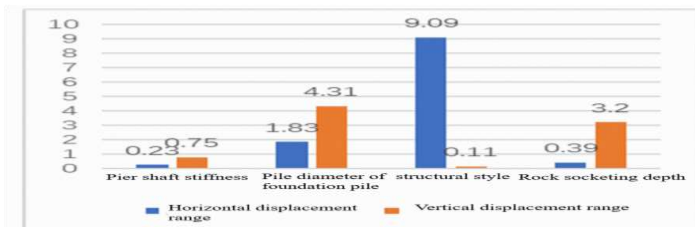
Figure 11: Analysis results of horizontal and vertical displacement of pier top
