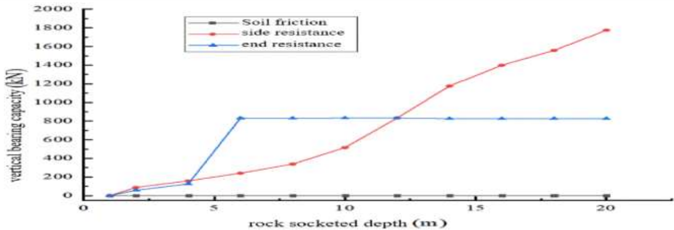
Figure 2: Distribution of vertical bearing capacity composition with rock socketed depth
