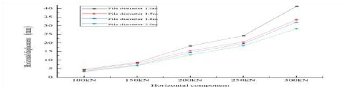
Figure 7 : Horizontal displacement of each pile diameter of pier 0
