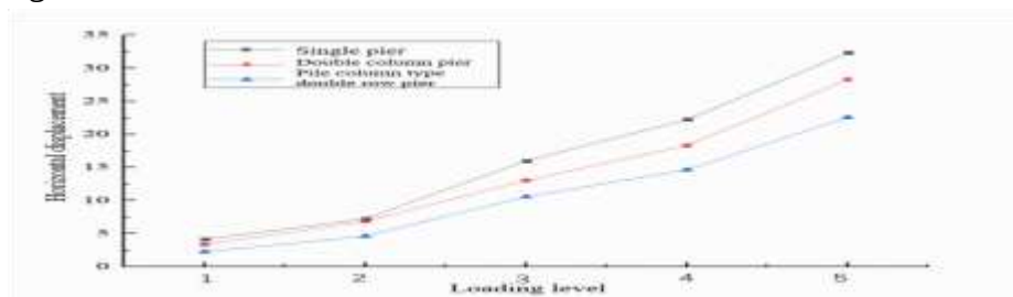
Figure 9: Horizontal displacement of various structural forms of pier 0
