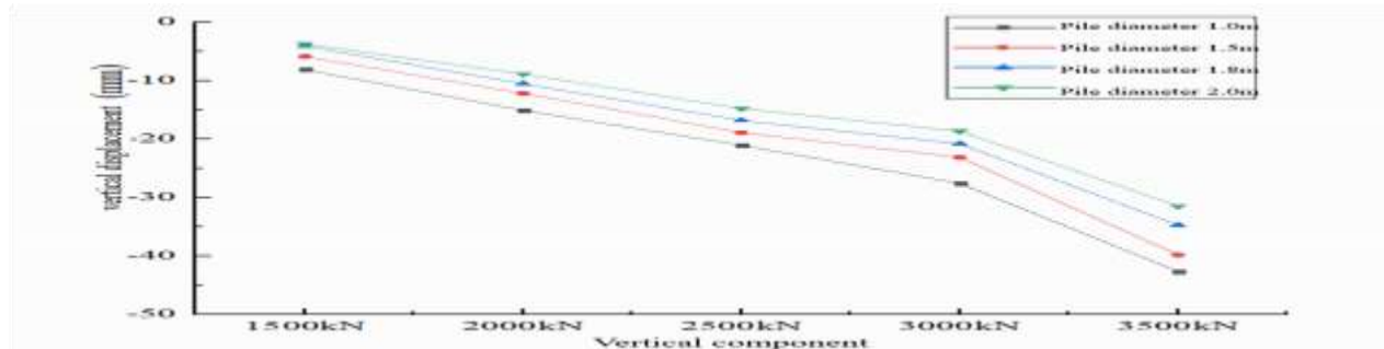
Figure 8 : Vertical displacement of each pile diameter of pier 0
