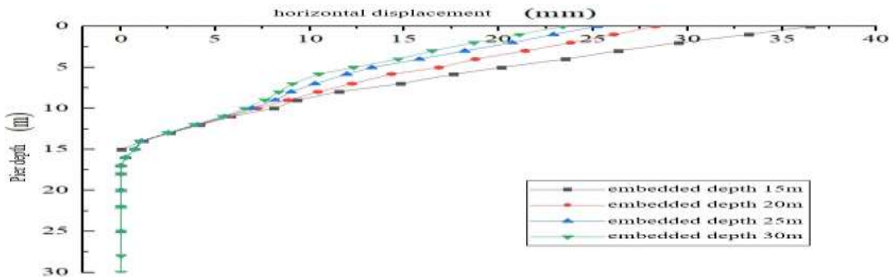
Figure 3: Influence of rock socketed depth change on horizontal displacement of pier
