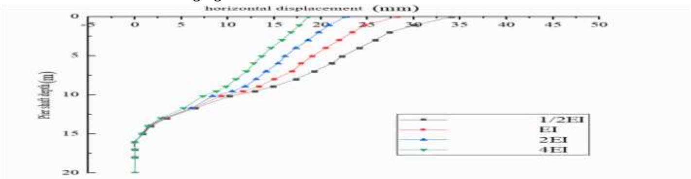
Figure 4: Effect of pier shaft stiffness on pier horizontal displacement
