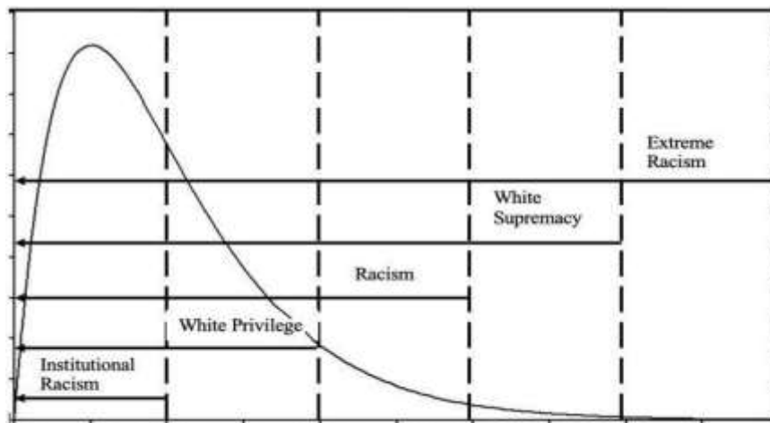
Figure 2, Racism as a Guttman Scale
