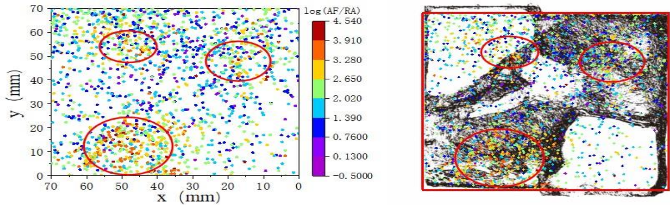
Figure 6: Comparison of projection of AE events localization points in coal samples
