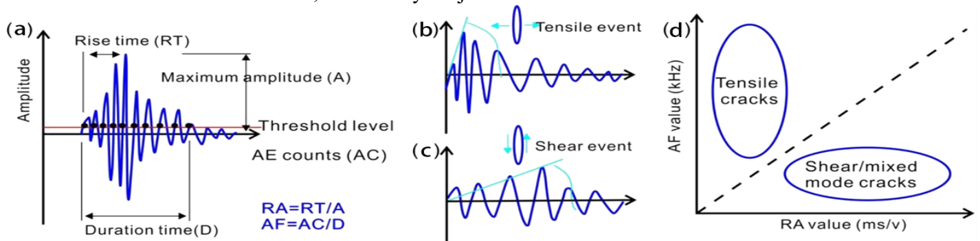
Figure 4: Typical AE wave forms of tensile and shear cracks [10]
