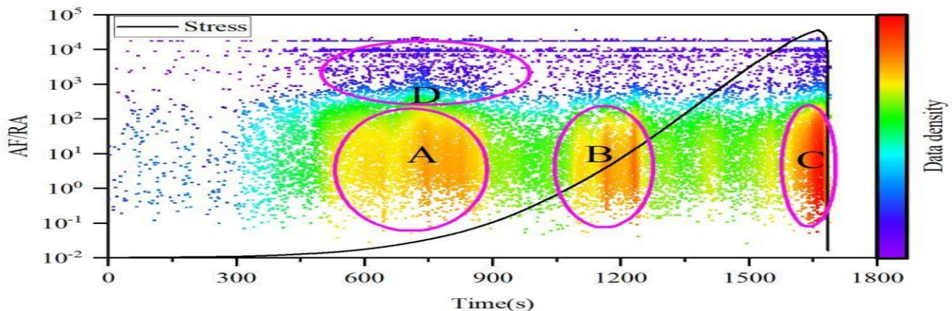
Figure 5: AF/RA characteristics of AE signals from coal samples
