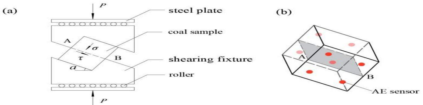
Figure 1: Schematic diagram of experimental method
