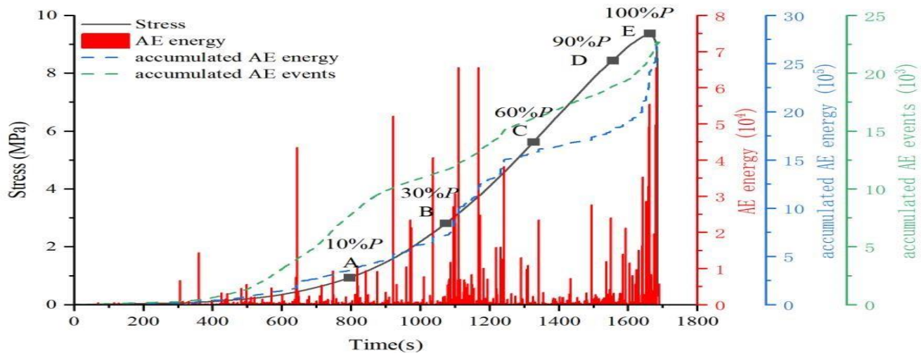
Figure 2: AE signals and stress curves
