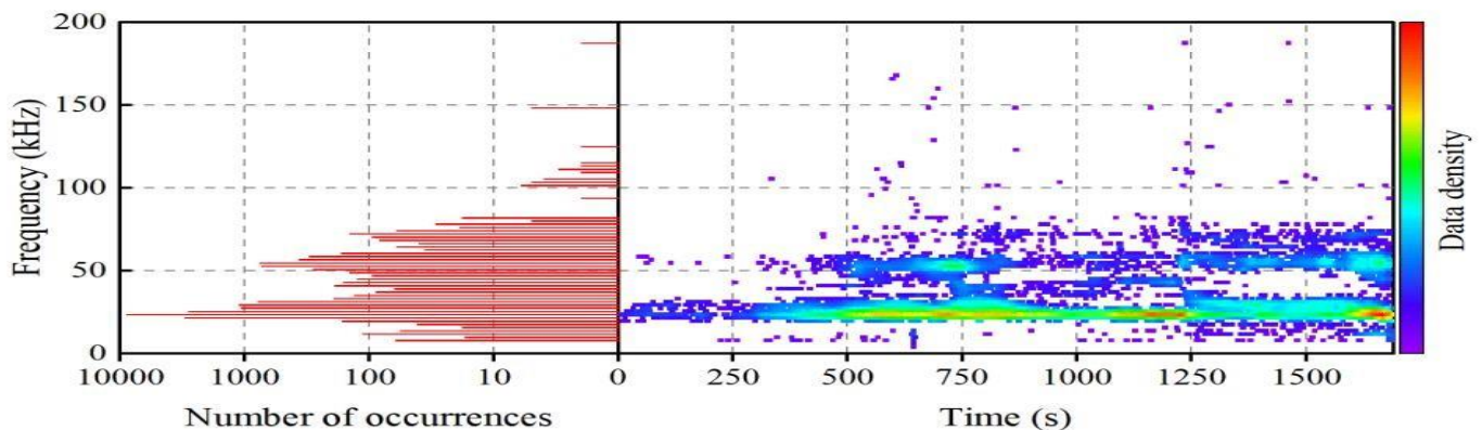
Figure 3: Frequency distribution of AE signals
