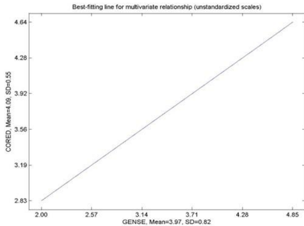
Figure 3: Relationship of GENSE and CORED Graphical Relationships among the Study Constructs
