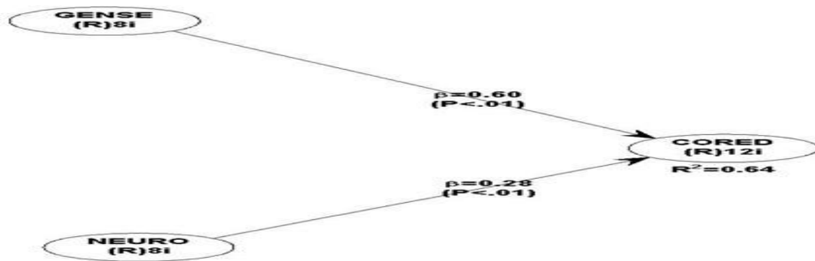
Figure 2: Assessment results for the structural model
