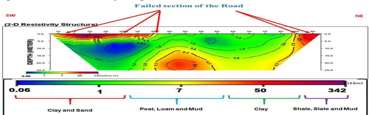
Figure 9: 2D Electrical Resistivity Tomogram for Profile QR
