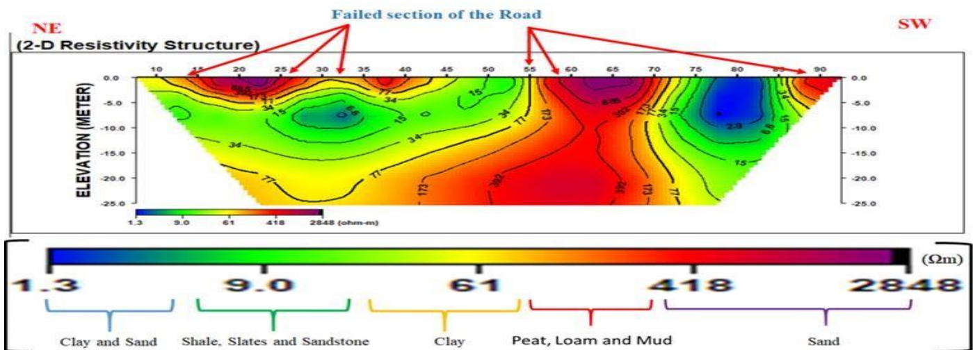
Figure 8: 2D Electrical Resistivity Tomogram for Profile MN.
