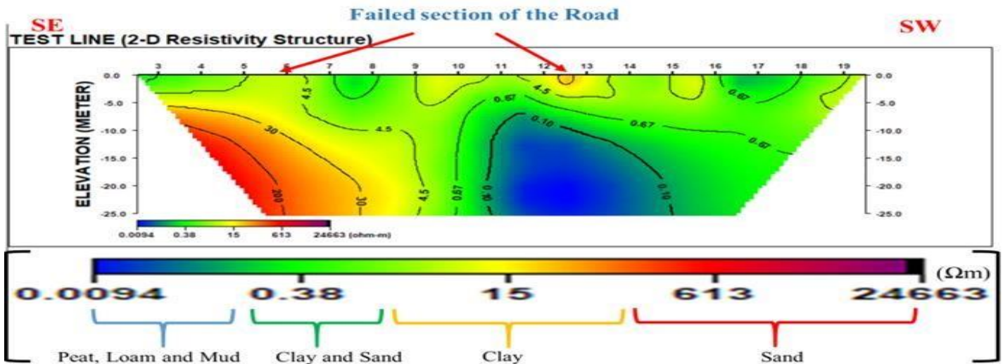
Figure 7: 2D Electrical Resistivity Tomogram for Profile CD
