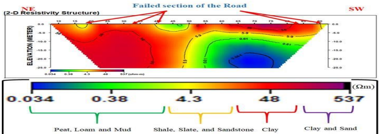
Figure 6: 2D Electrical Resistivity Tomogram for Profile AB.
