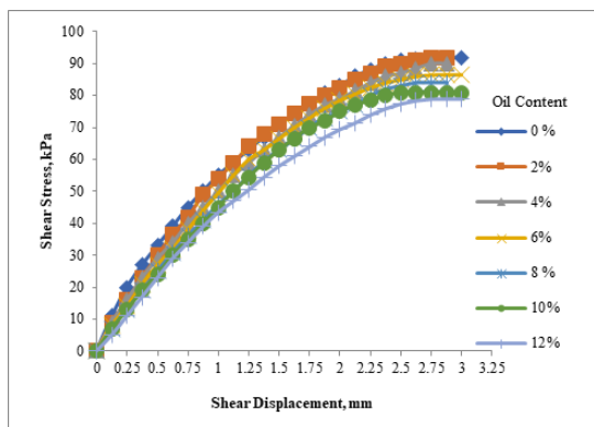
Figure 23: 45 Days Aging Effect Curve of Shear Stress vs. Shear Displacement for Lubricated Loose Sand at 150 kPa Normal Stress
