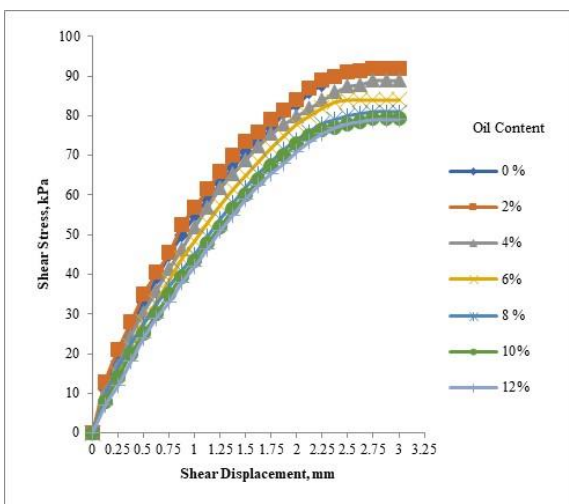
Figure 17: 30 Days Aging Effect Curve of Shear Stress vs. Shear Displacement for Contaminated Loose Sand at 100 kPa Normal Stress
