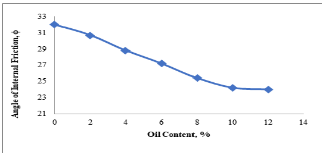
Figure 15: Effect of Oil Content on the Variation of Angle of Internal Friction
