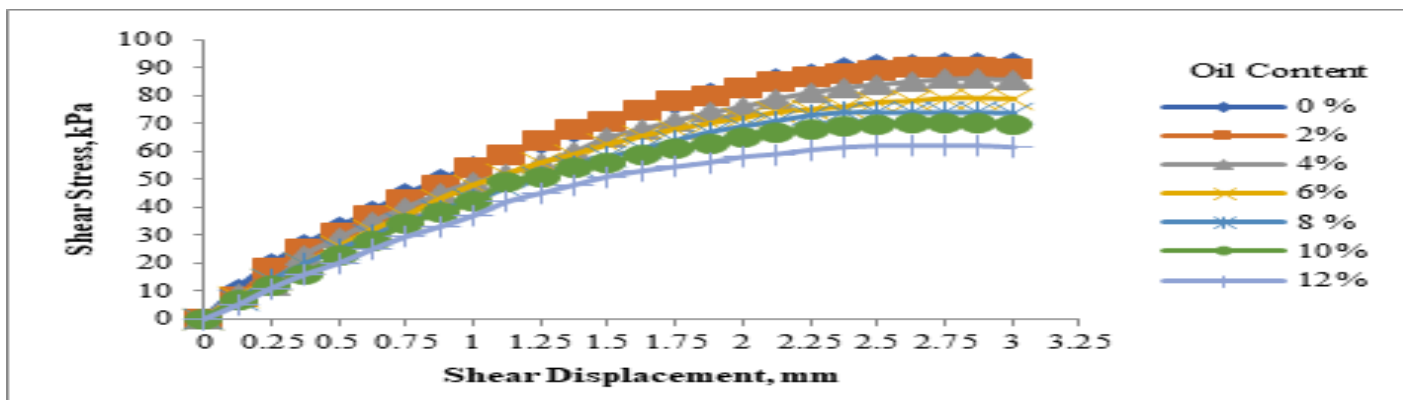
Figure 3: Immediate Response Curve of Shear Stress vs. Shear Displacement for Contaminated Loose Sand at 150 kPa Normal Stress
