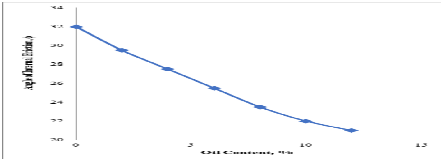
Figure 5: Effect of Oil Content on the Variation of Angle of Internal Friction
