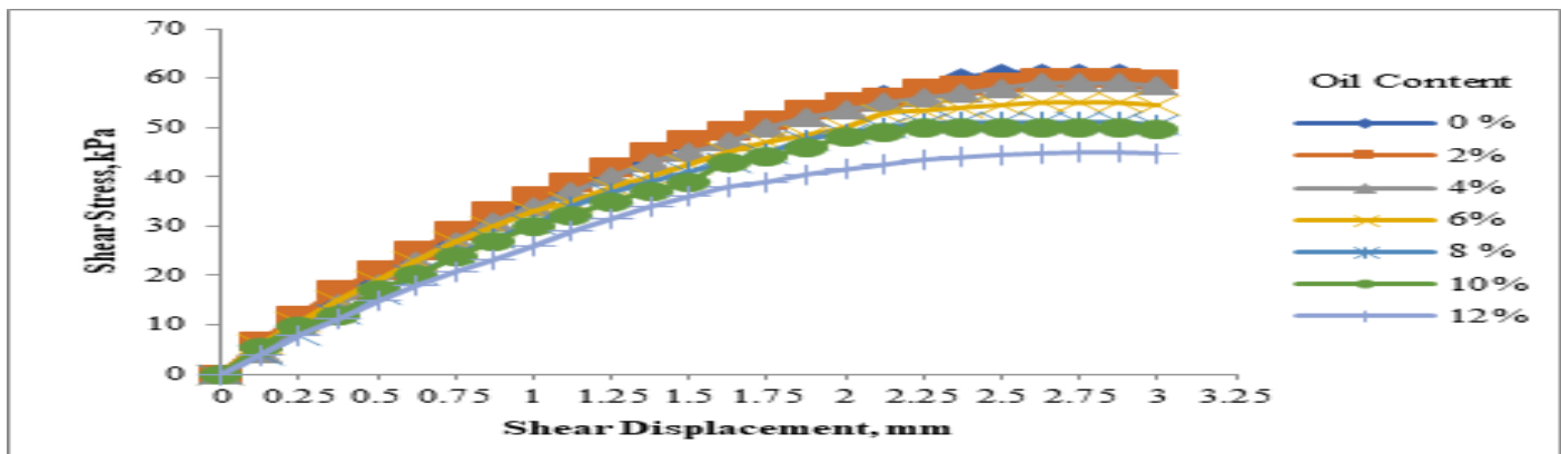
Figure 2: Immediate Response Curve of Shear Stress vs. Shear Displacement for Contaminated Loose Sand at 100 kPa Normal Stress
