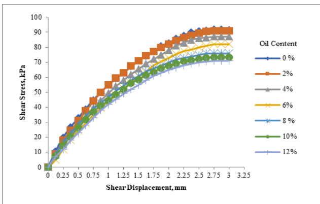
Figure 13: 15 Days Aging Effect Curve of Shear Stress vs. Shear Displacement for Contaminated Loose Sand at 150 kPa Normal Stress
