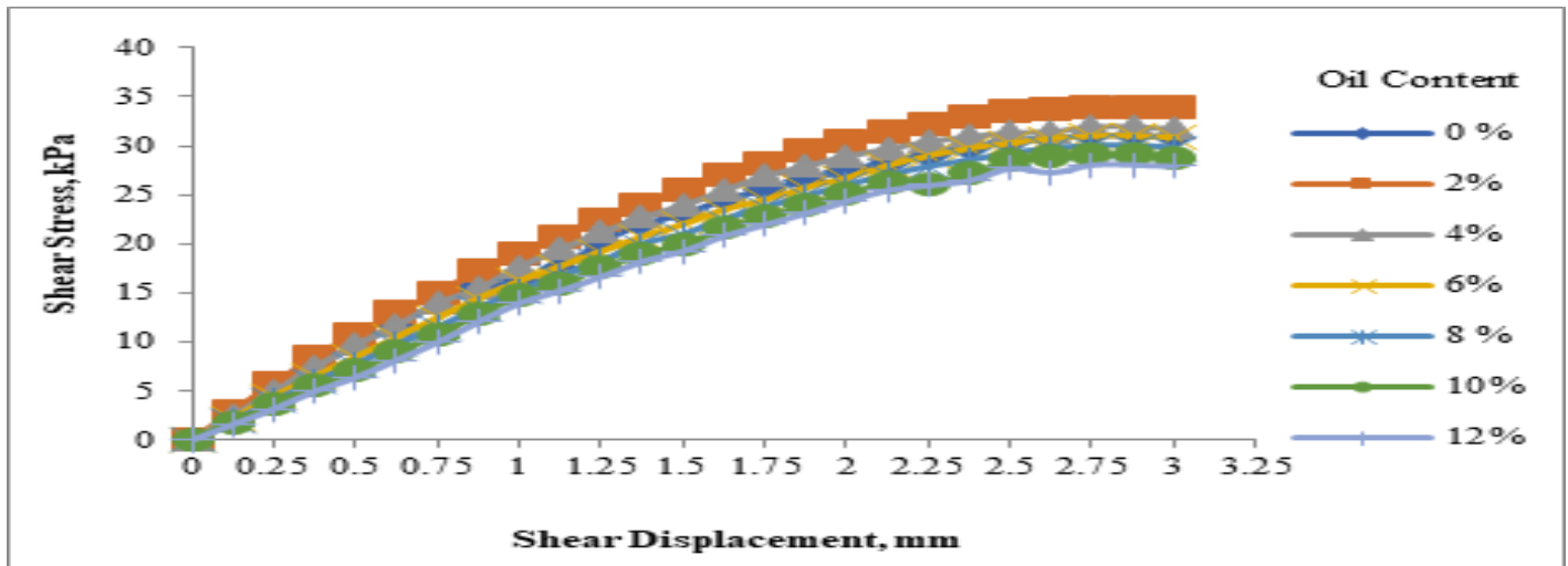
Figure 1: Immediate Response Curve of Shear Stress vs. Shear Displacement for Contaminated Loose Sand at 50 kPa Normal Stress
