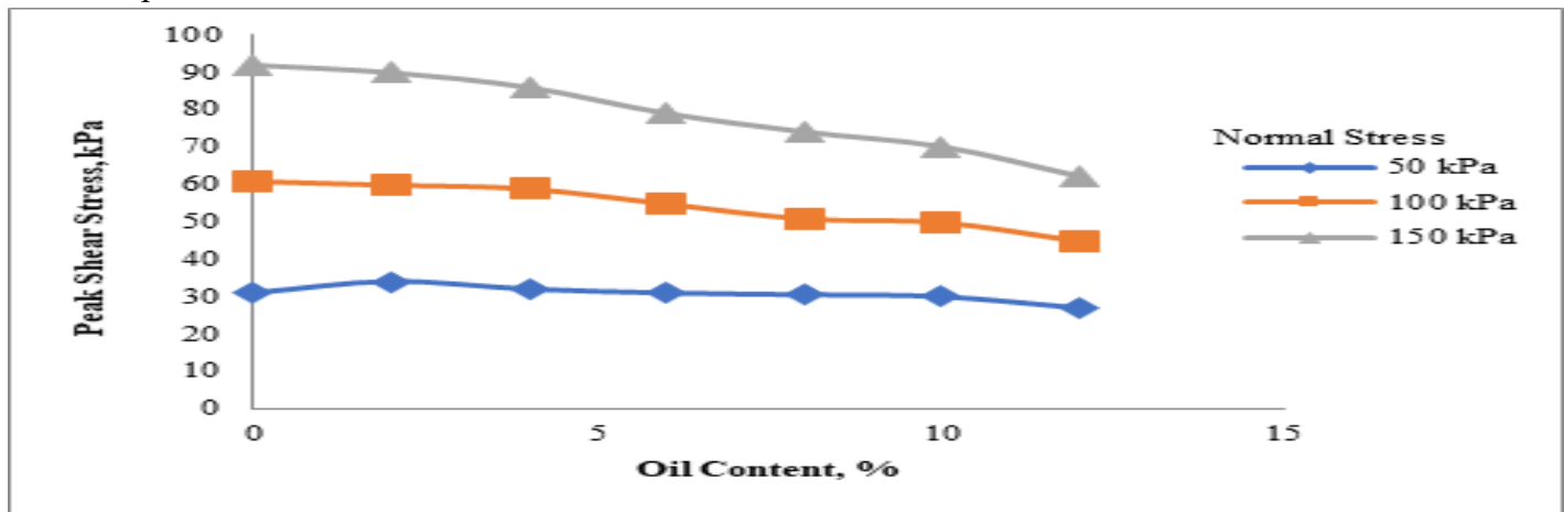
Figure 4: Variation of Ultimate Shear Stress with Respect to Varying % of Oil Content
