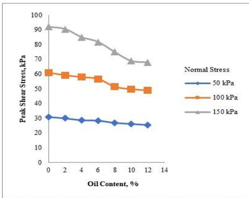
Figure 9: Variation of Peak Shear Stress with Respect To Varying % of Oil Content
