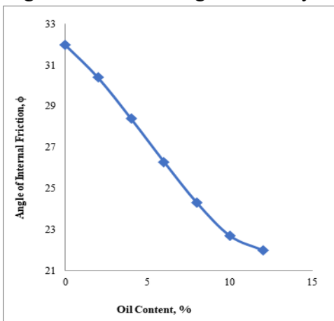
Figure 10: Effect of Oil Content on the Variation of Angle of Internal Friction
