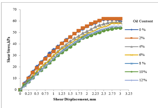
Figure 17: 30 Days Aging Effect Curve of Shear Stress vs. Shear Displacement for Contaminated Loose Sand at 100 kPa Normal Stress
