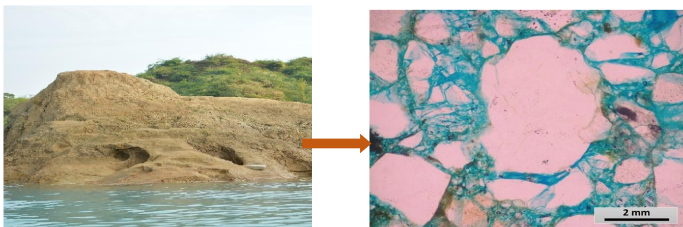
Fig. 8. Photomicrograph showing the thin section of a conventional reservoir with 18 to 20% porosity range.
