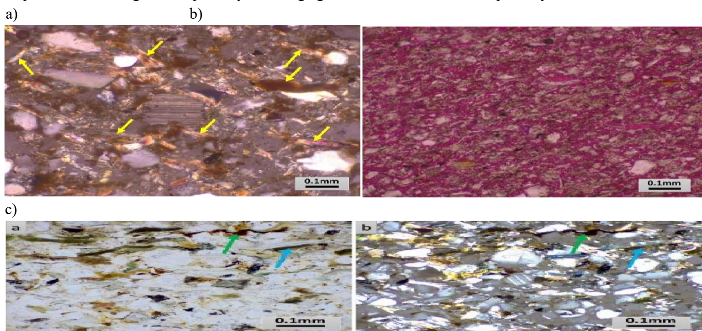
Fig. 9. These photomicrographs represent a) Compaction, b) cementation, and c) chlorite rims.
