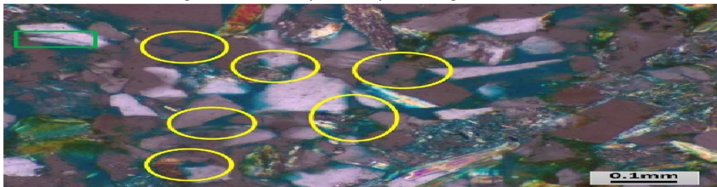
Fig. 10. Photomicrograph exhibiting porosity enhanced by dissolution (yellow circle) and fracturing (green rectangle).
