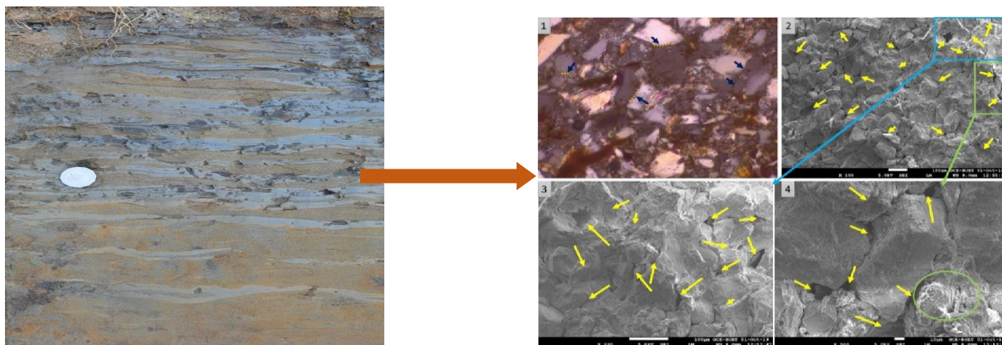
Fig. 7. A tight gas sandstone with an average porosity of 7 to 8%. In addition, dissolution porosity enhances reservoir quality here.
