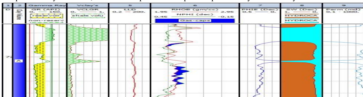
Figure 6: Compartmentalization within reservoir A showing the two compartments with gas caps in blue.
