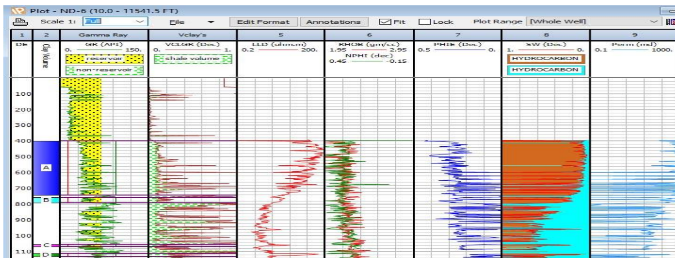
Figure 5: log signatures of Vsh, porosity, permeability, water and hydrocarbon saturation for well ND-6
