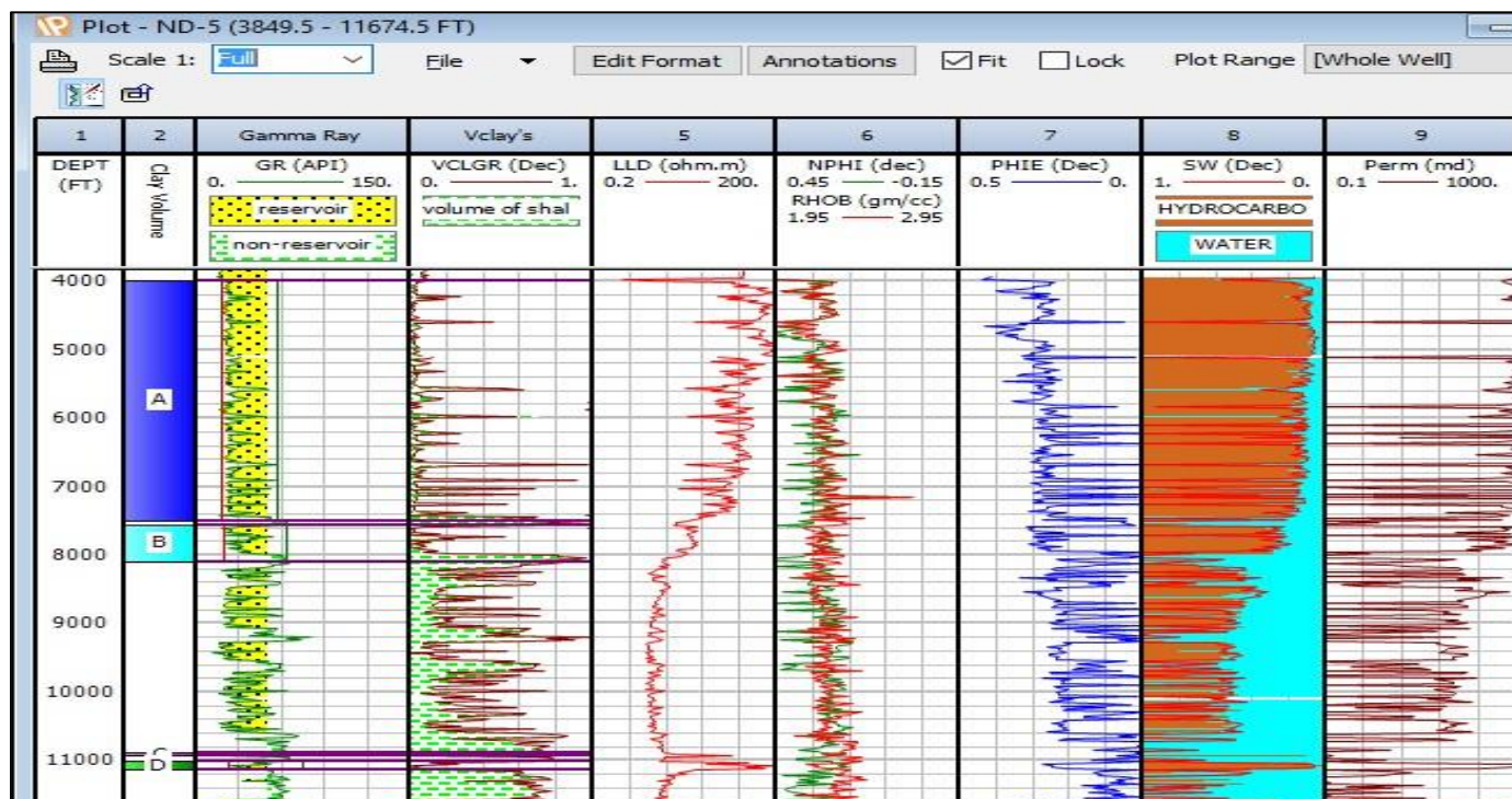
Figure 3: Log signatures of Vsh, porosity, permeability, water and hydrocarbon saturation of well ND-5
