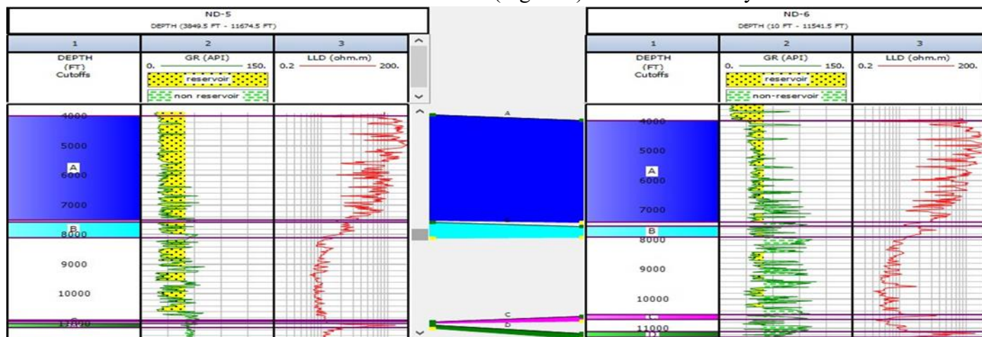
Figure 2: Correlated reservoirs across wells ND-5 and Well ND-6
