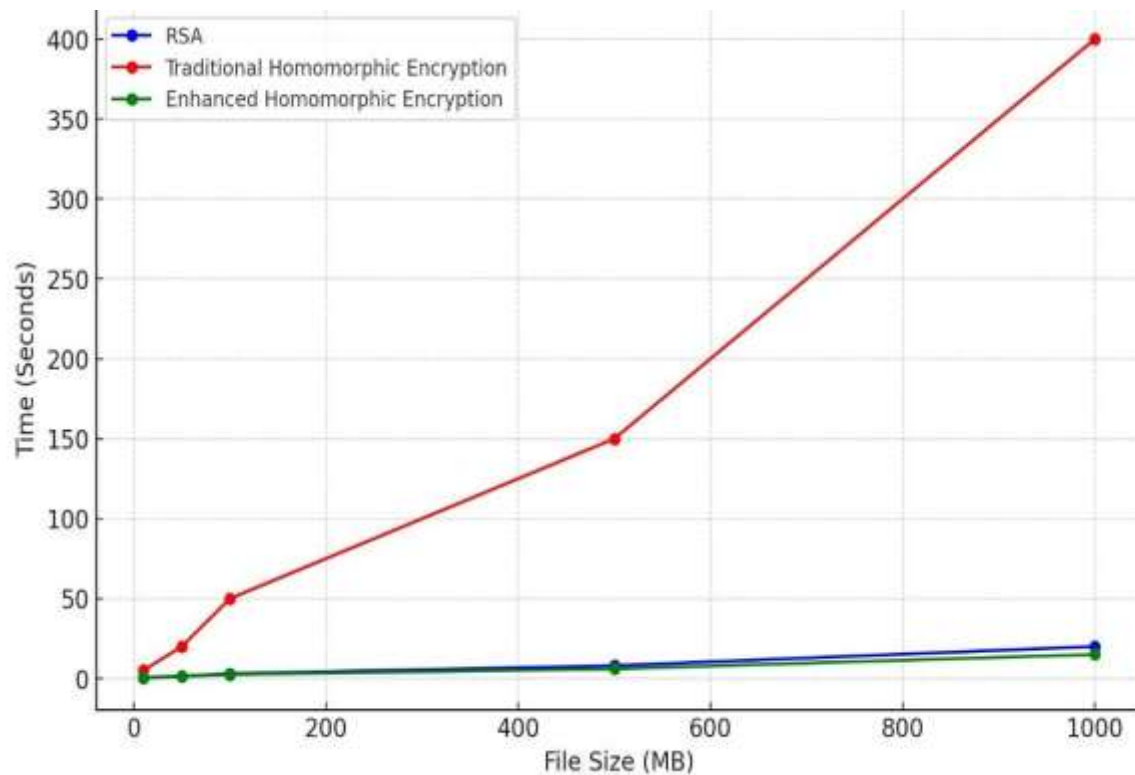
Figure 1: Graph of Time Complexity of RSA, HE and EHE
