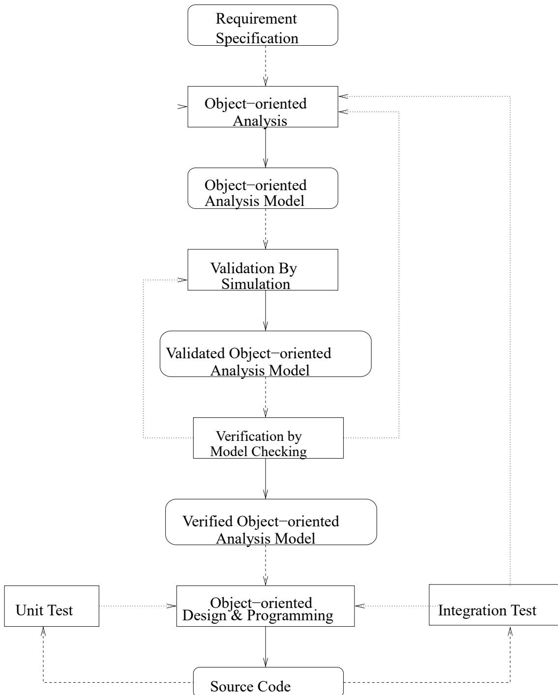
Figure 2: Integration of Model Checking and Object-Oriented Software Development Process
