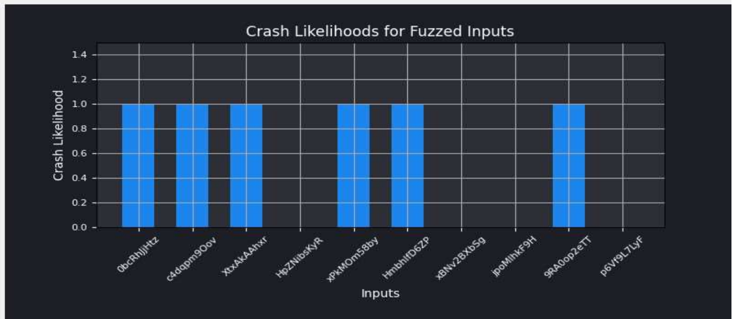
Figure 9: Crash Likelihoods for Fuzzed Inputs Model Checking Integration
