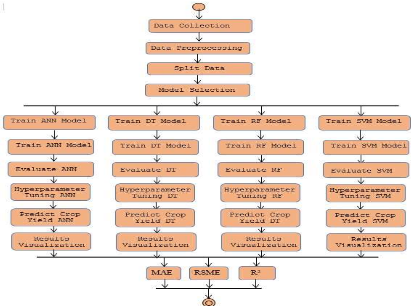
Figure 2: The activity diagram depicting the flow of tasks and decisions in the crop yield prediction process.
