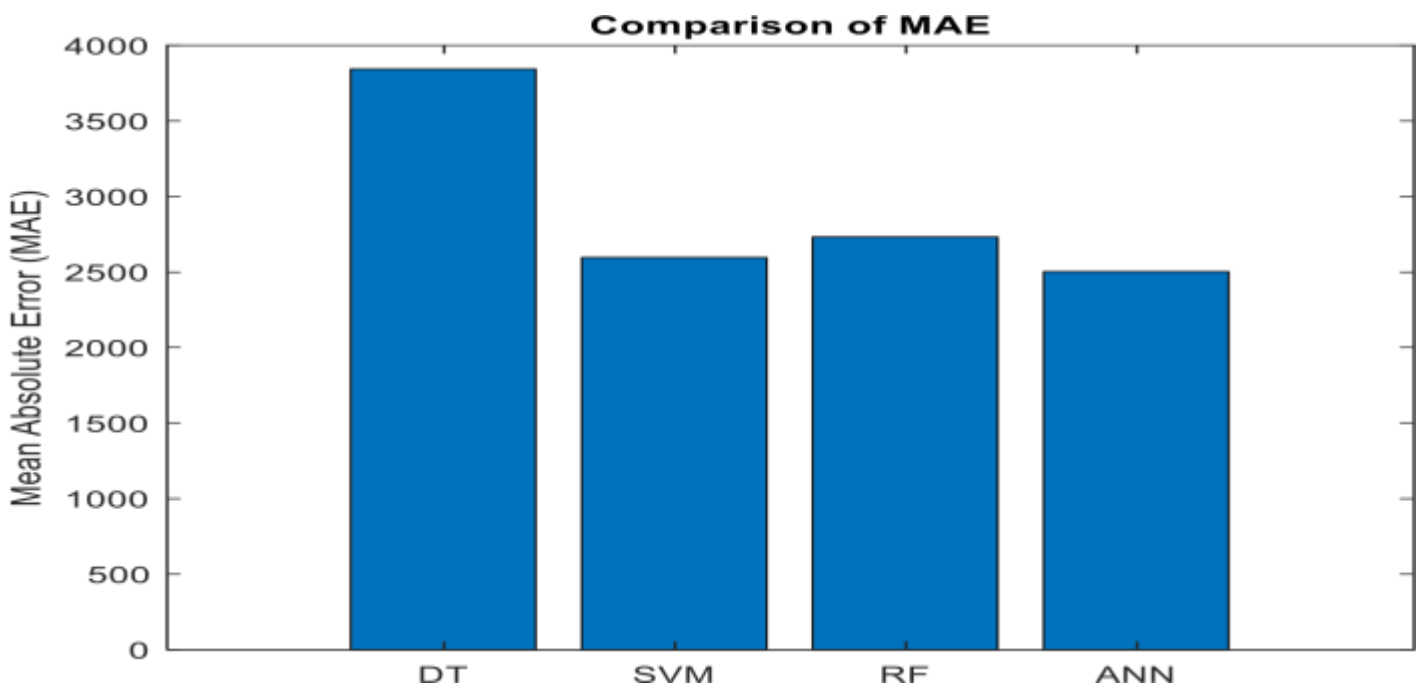
Figure 4 visualizes a comparison of the MAE of the models
