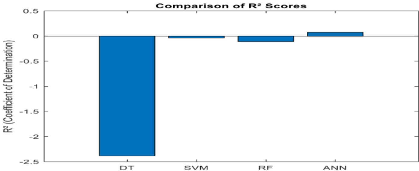
Figure 5 visualizes a comparison of the R^2 of the models
