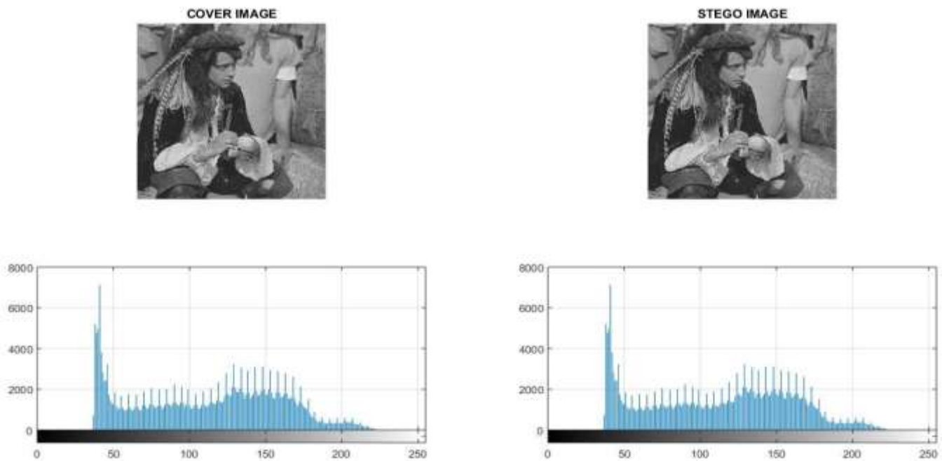
Figure 4.11: Result for Cover image Pirate, its Stego image and corresponding Histograms
