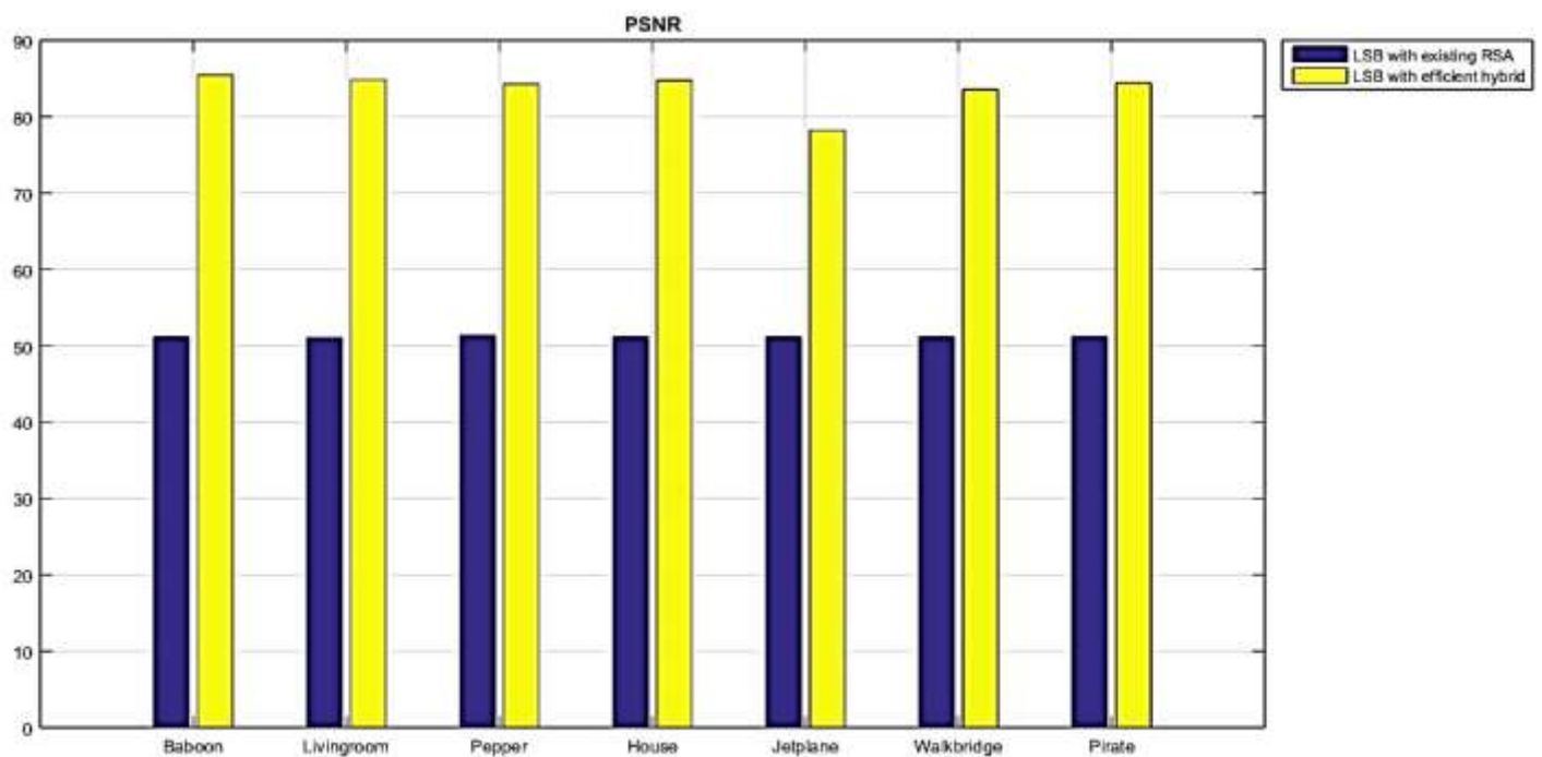
Figure 4.13: Graph showing PSNR values for LSB with RSA and LSB with hybrid (modified) RSA
