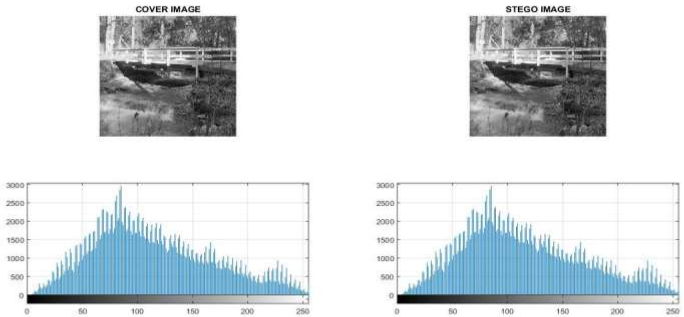
Figure 4.10: Result for Cover image Walk bridge, its Stego image and corresponding Histograms
