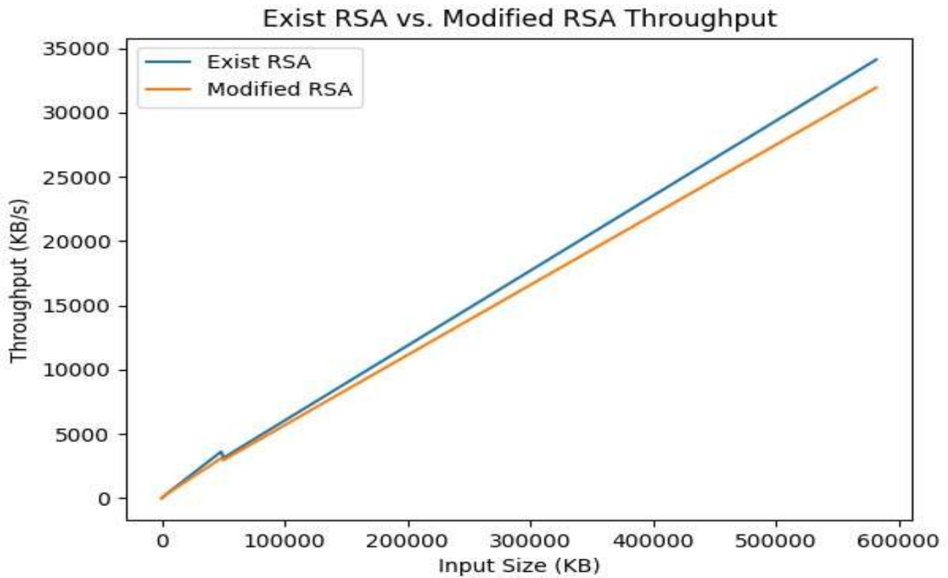
Figure 4.4: Throughput for the Existing RSA vs Hybrid RSA Decryption
