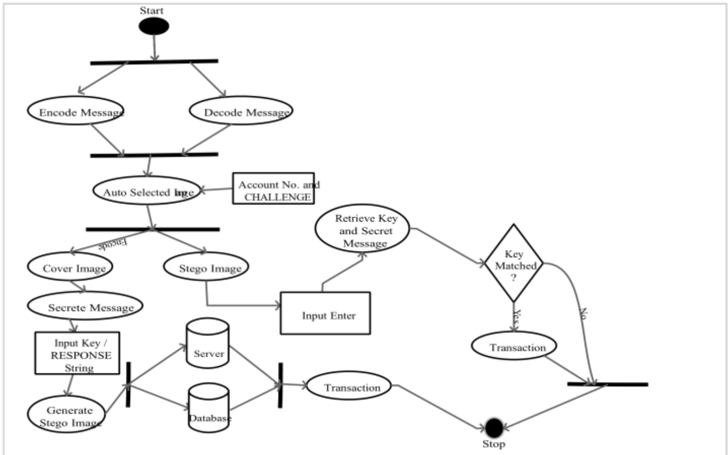
Figure 3.3: Activity Diagram for the system
