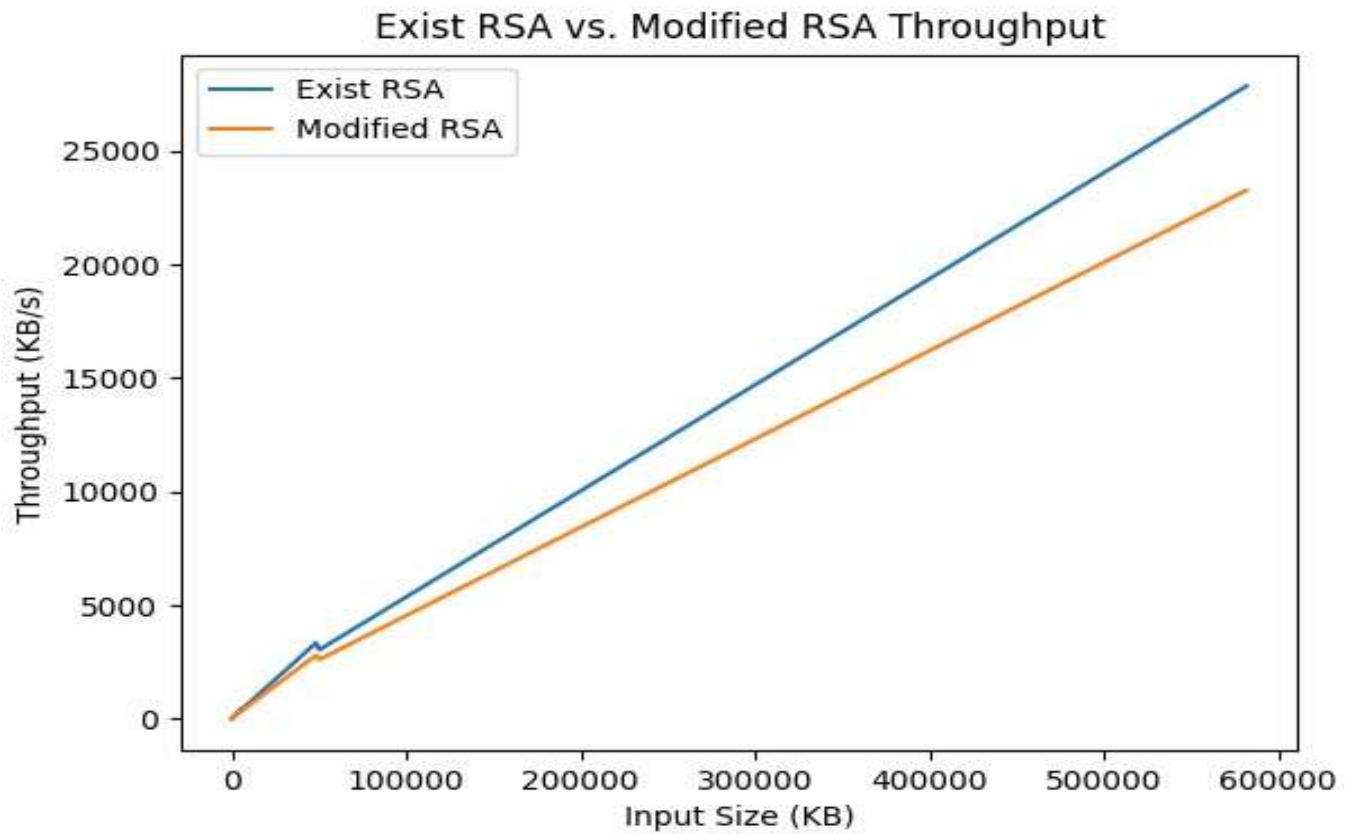
Figure 4.3: Throughput for the Existing RSA vs Hybrid RSA Encryption
