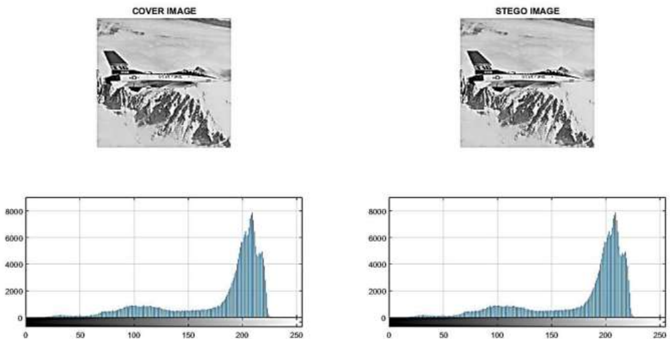
Figure 4.9: Result for Cover image Jet plane, its Stego image and corresponding Histograms
