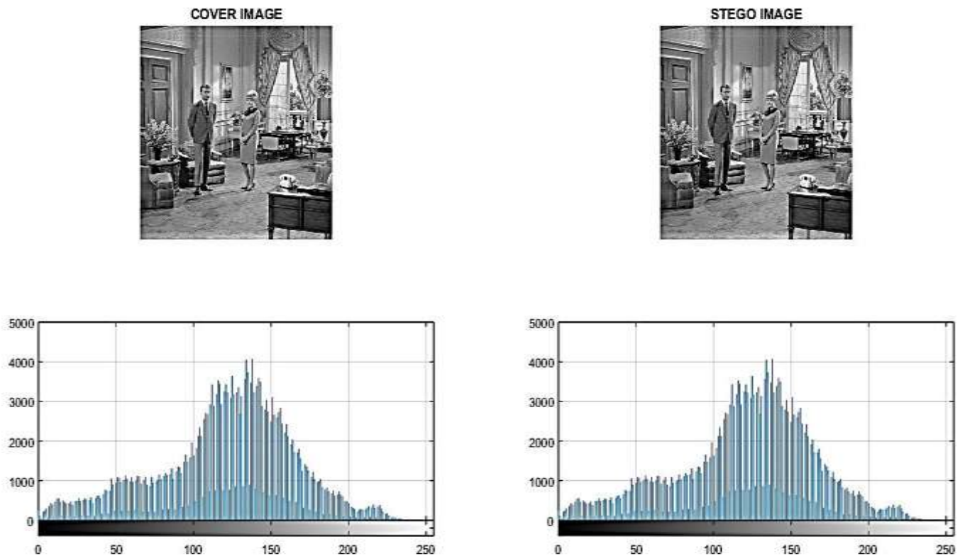
Figure 4.6: Result for Cover image Livingroom, its Stego image and corresponding Histograms.
