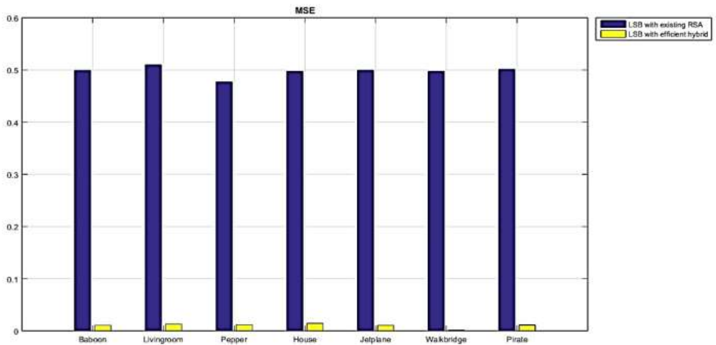
Figure 4.12: Graph showing MSE values for LSB with RSA and LSB with hybrid (modified) RSA
