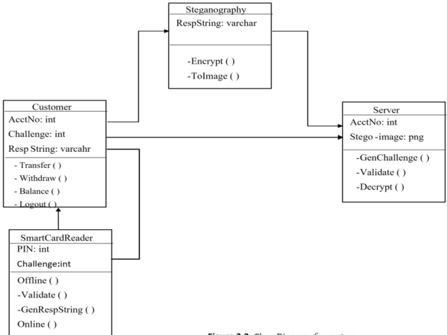
Figure 3.2: Class Diagram for system
