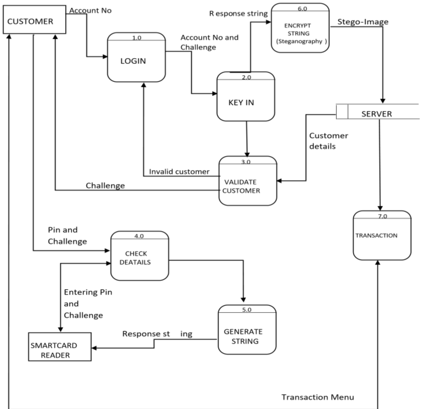
FIGURE 3.4: Data Flow Diagram for System Existing RSA calculation.
