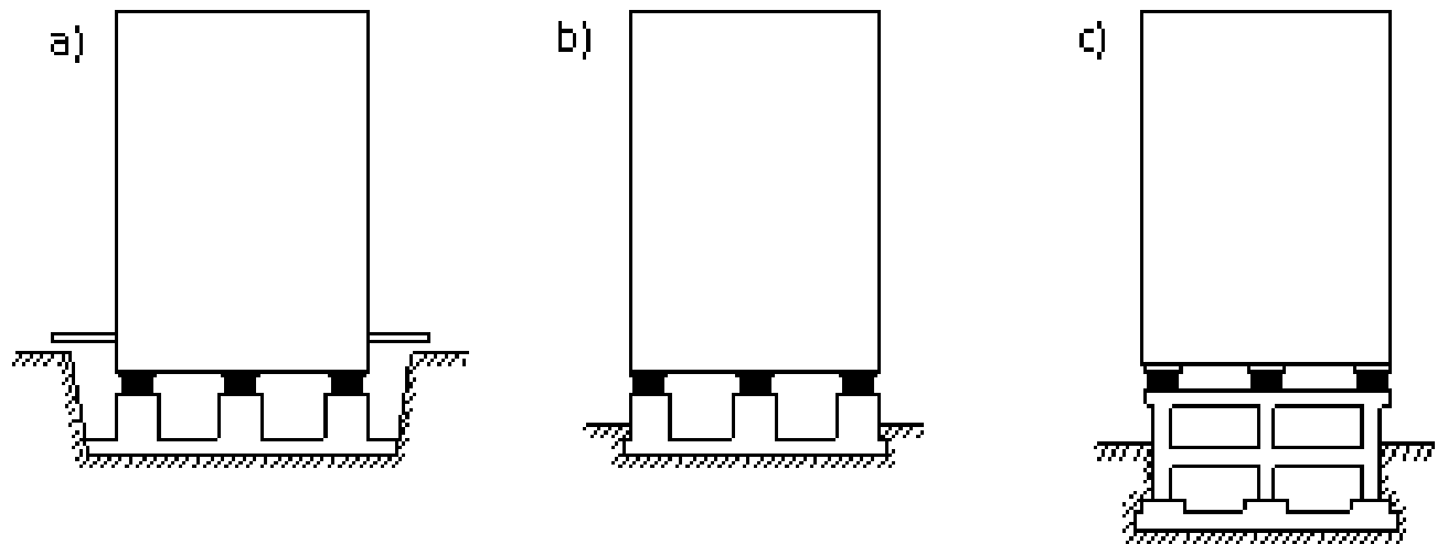
Figure 1. Main types of location of seismic isolation systems
