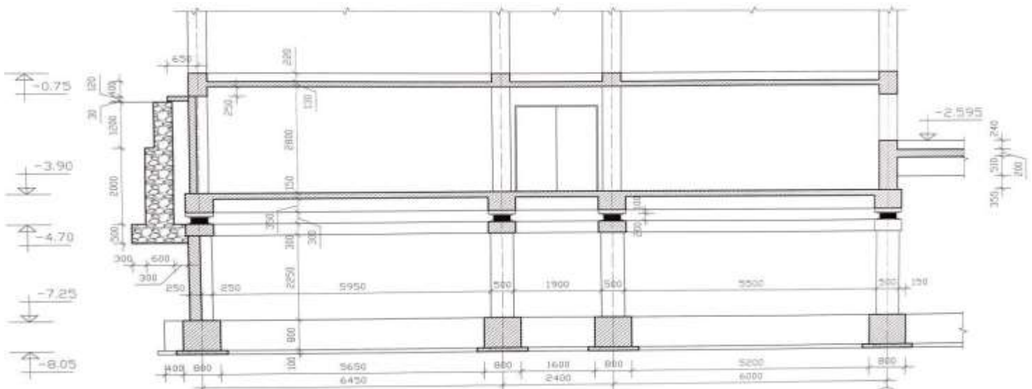
Figure 4. Vertical elevation of the isolation system between the axes “1” and “11”
