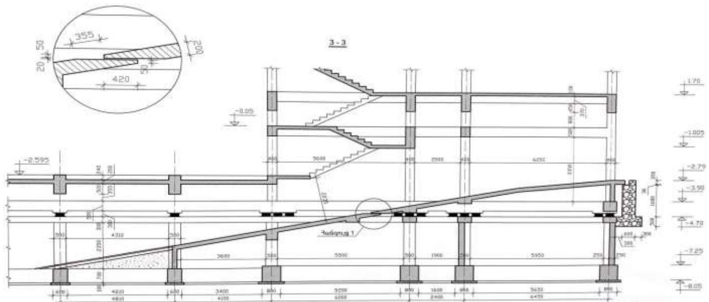
Figure 5. Vertical elevation of the isolation system along the inclined slab of the entrance to the parking floor
