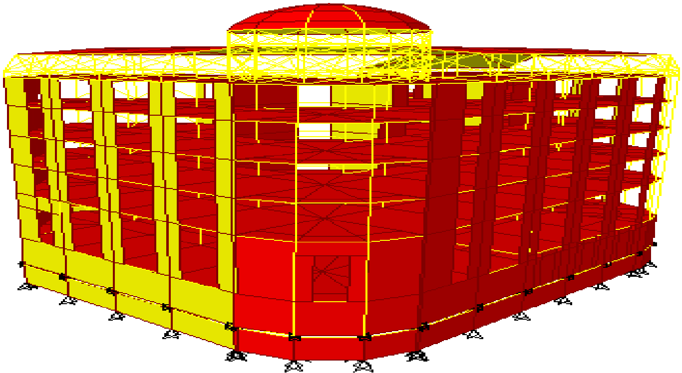
Figure 6. Design model of the 7-story base isolated “Tufenkian” building with non-symmetric plan of the multifunctional hotel/commercial center complex constructed in Yerevan
