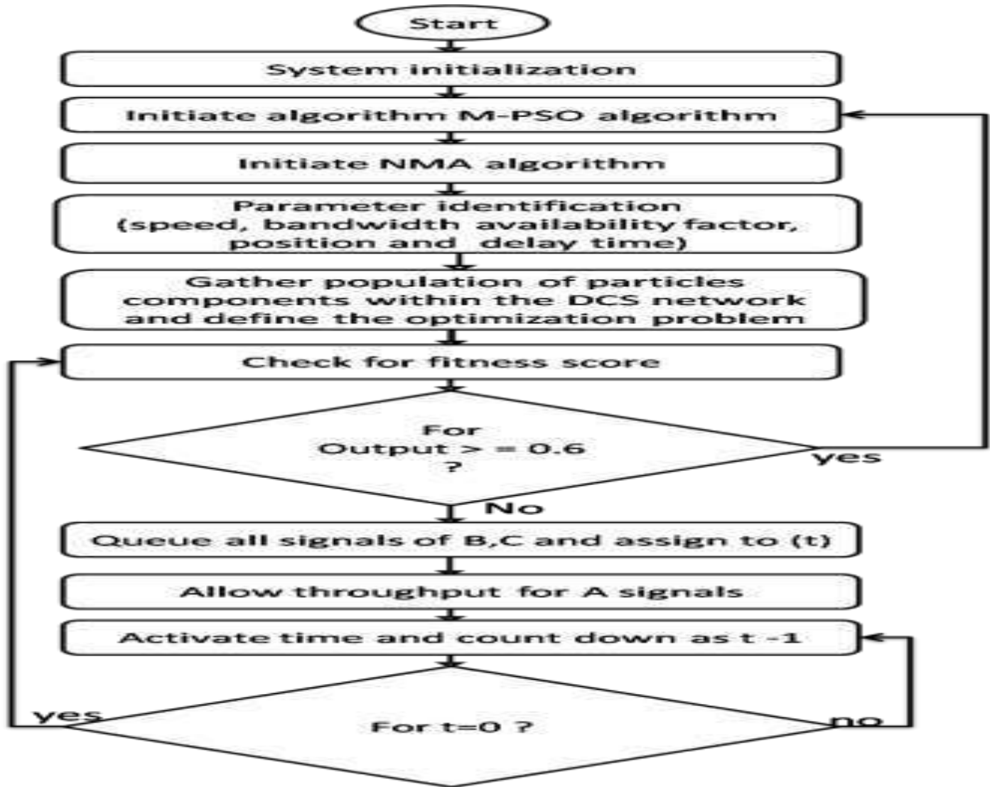
Figure 2: Flowchart of the model for management of communication delay
