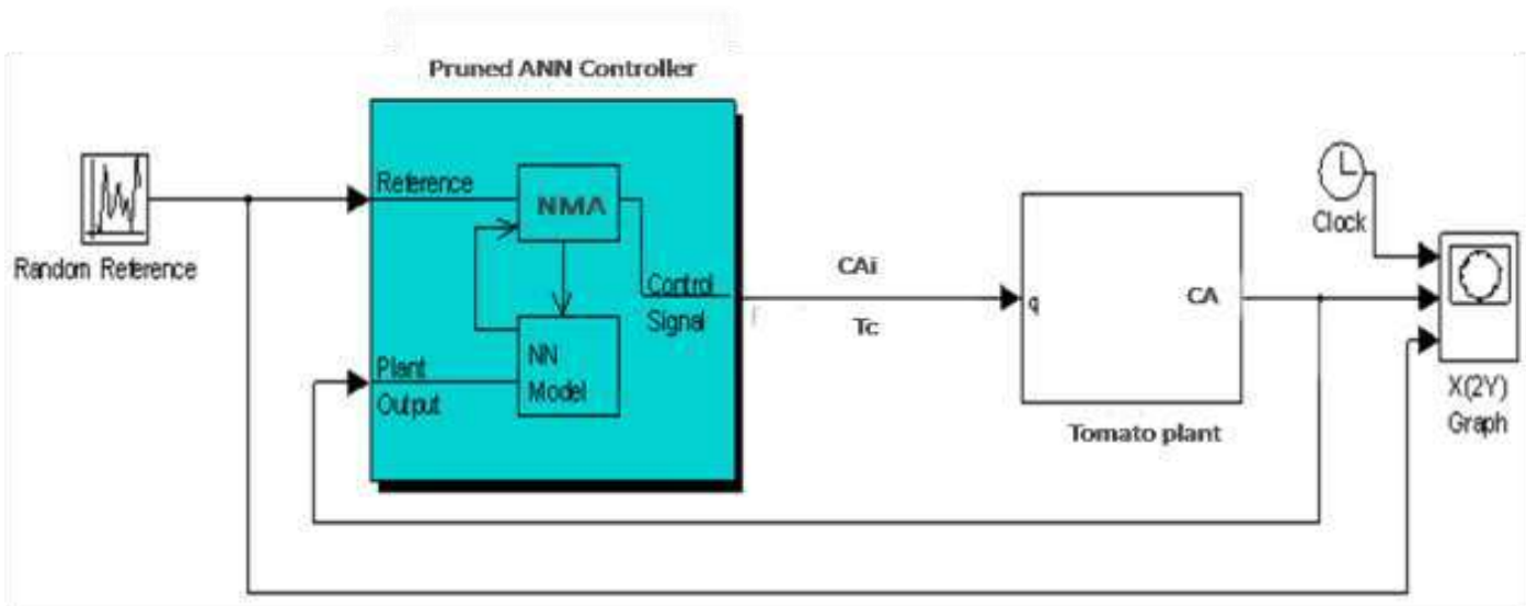
Figure 4: Simulink of the neural network control system
