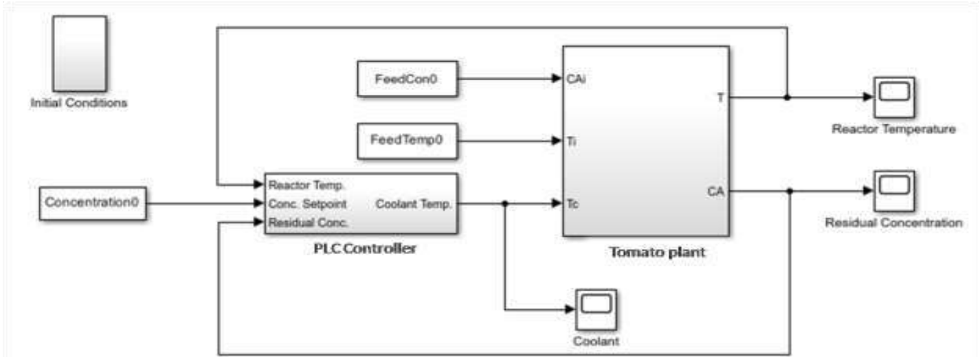
Figure 3: Simulink of the PLC control system
