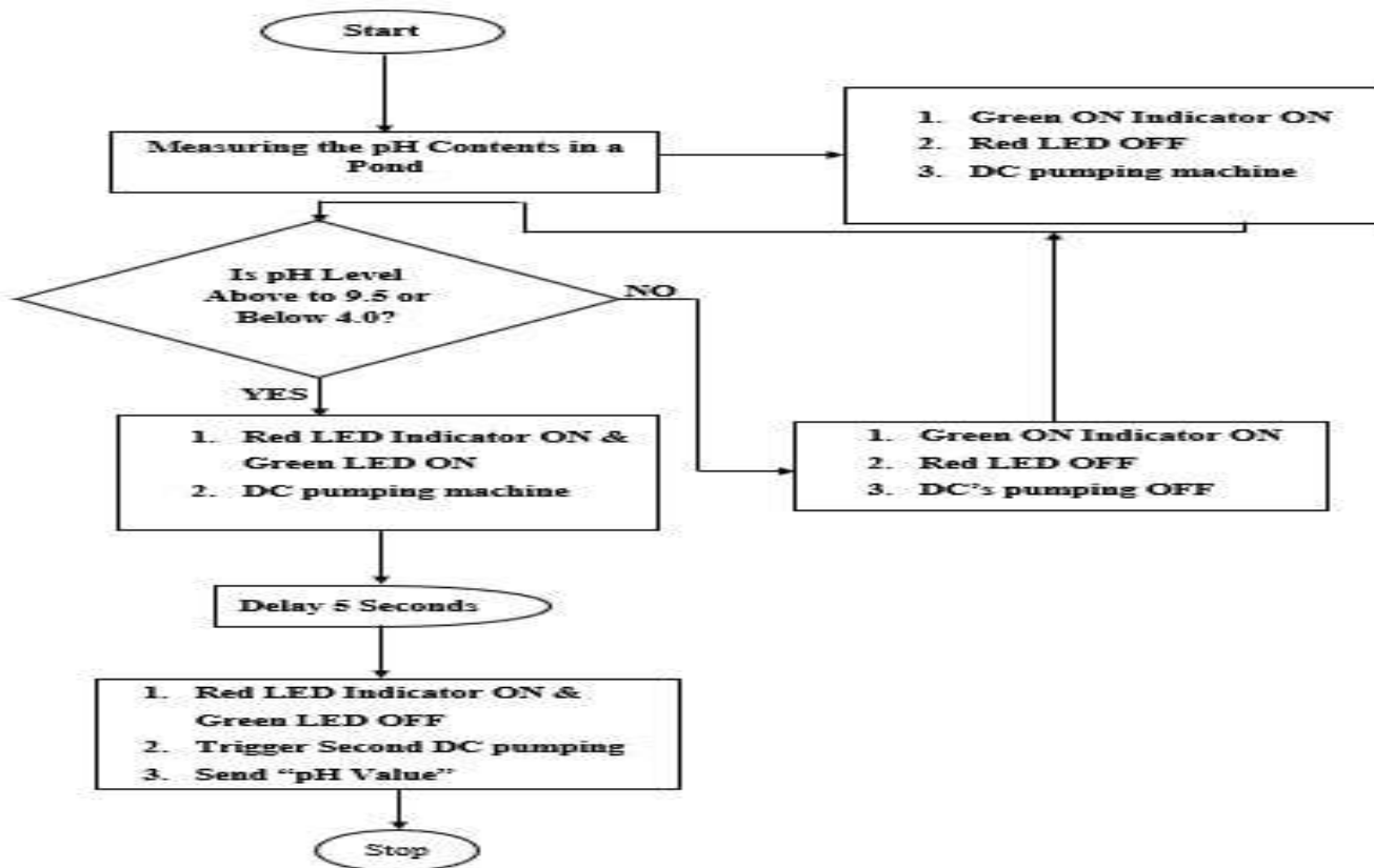
Figure 13: Flowchart of the IOT based integrated water quality monitoring device
