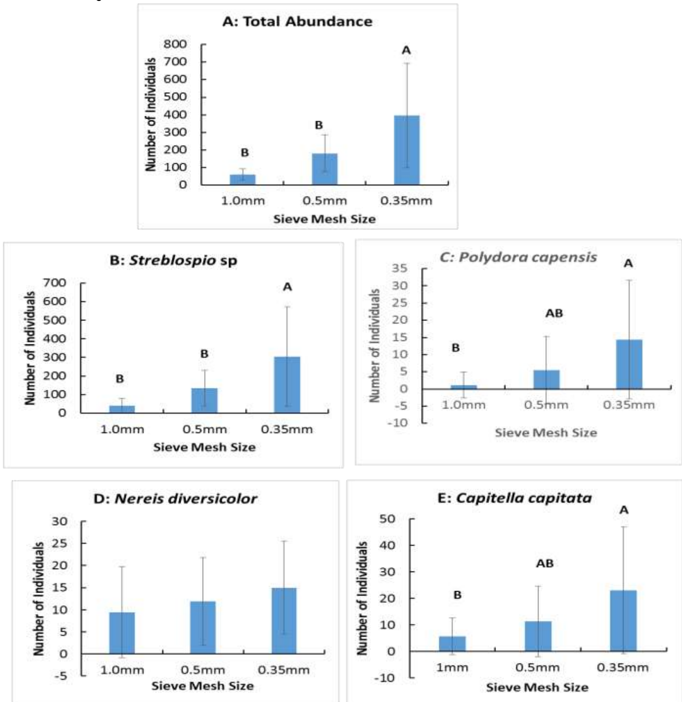
Fig 3. Abundance of Macrobenthic Fauna Mean (Mean \pm SD, n= 12) from Three Sieve Mesh Sizes in Obufe Creek. Means with different alphabets are significantly different (Tukey, p < 0.05 ).
