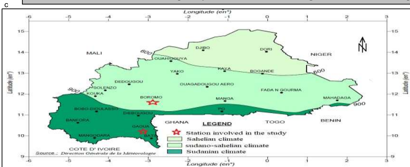
Figure 2: Location of the synoptic stations considered in the study
