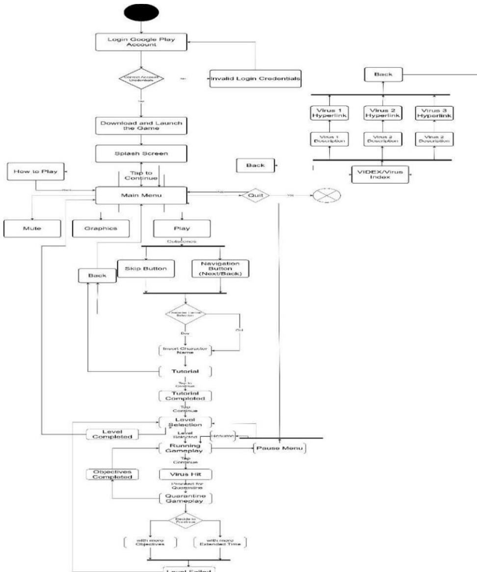
Figure 3. Activity Diagram of Virus Evasion Development
