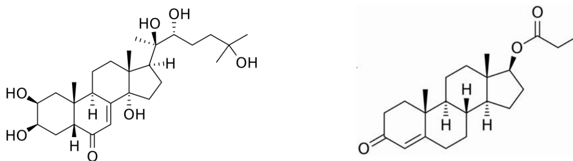
Fig. 1. Structure of 20-HE and testosterone propionate (TP). 20-HE is a structural analogue of TP.
