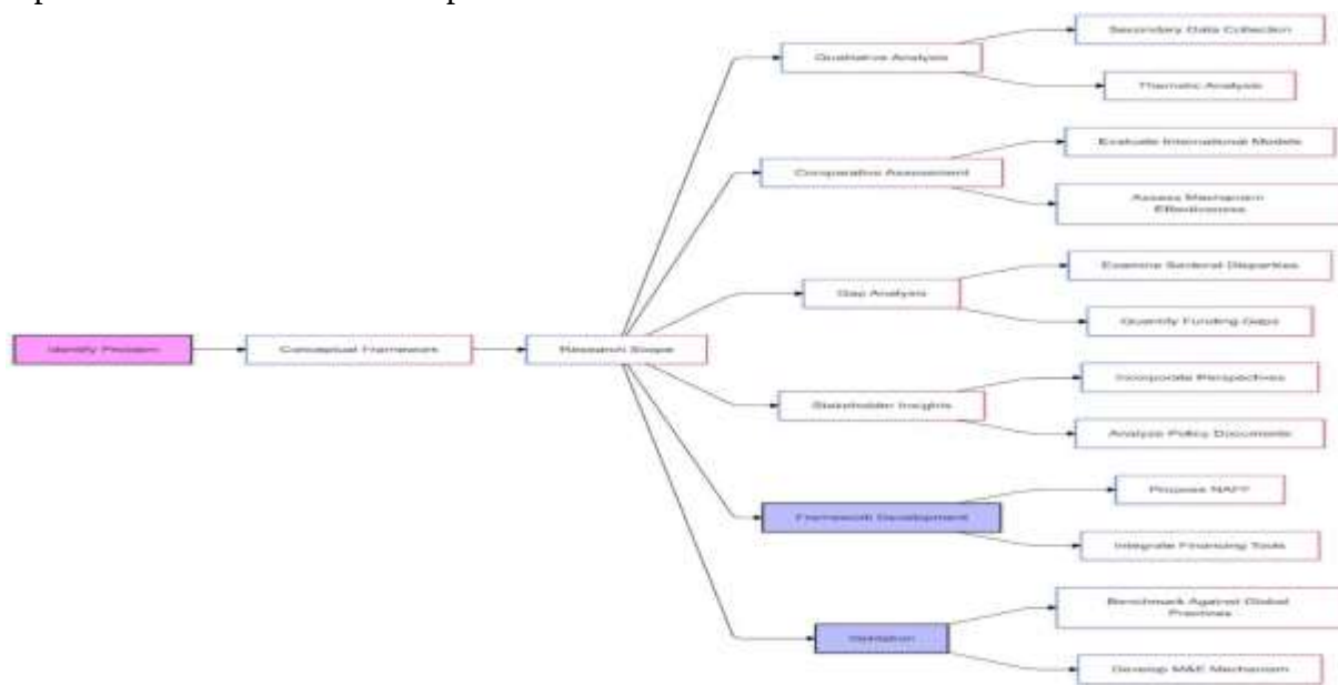
Figure 1: Methodology.
