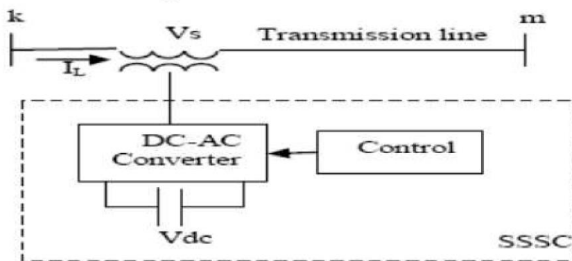
Figure 2: .Basic Configuration of Static Synchronous Series Compensator
