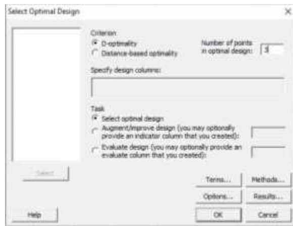
Figure 10. Selection of the optimal design from the Select Optimal Design dialog box.
