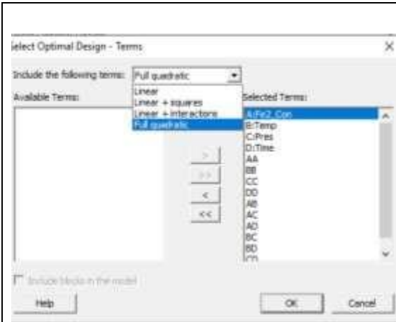
Figure 11. Selection of the optimal design probable model (Full Quadratic) from the Select Optimal Design-Terms dialog box.
