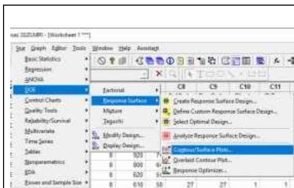
Figures 15. Selection of Contour/Surface Plots through STAT, DOE and RESPONSE SURFACE.
