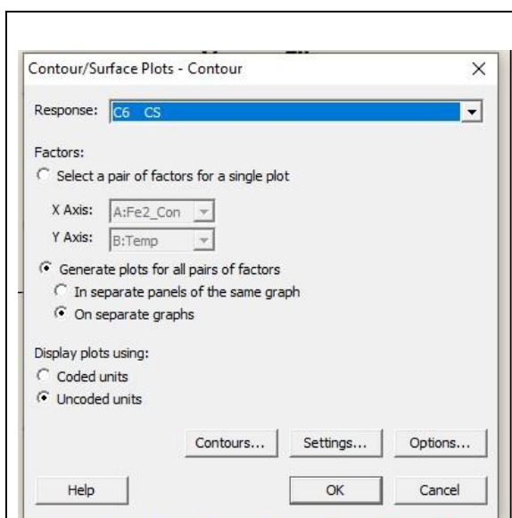
Figures 17. Setup of the contour plots from the dialog-box of Contour/Surface-Contour Plots.
