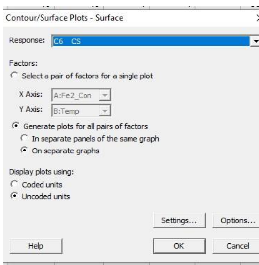
Figures 18. Setup of the surface plots from the dialog-box of Contour/Surface-Surface Plots.
