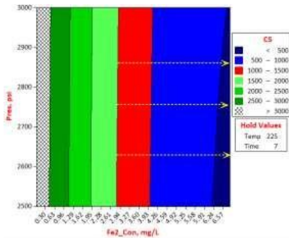
Figure 23. A 3D Contour Plot of CS vs Pres., and Fe2_Con., at Constant Temp. (225°F) and Time (7hrs); which Shows the Optimal Zone, Comfort Zone, and Adverse Zone of Compressive Strength in a Ferrous Cement Sheath System.
