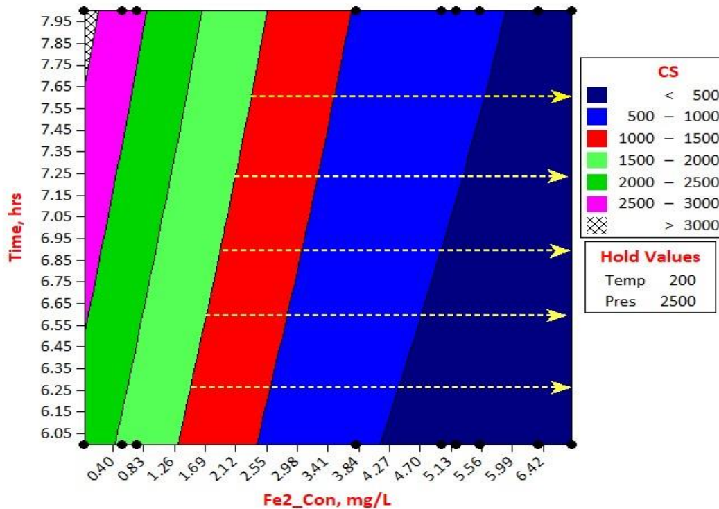
Figure 27. The Optimal Zone, Comfort Zone, and Adverse Zone of Compressive Strength in a Ferrous Cement Sheath System; which is depicted in the 3D Contour Plot of CS vs Time, and Fe2_Con., at Constant Temp. (200°F) and Pres. (2500psi).
