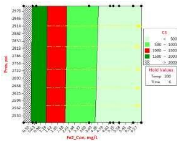
Figure 26. The Optimal Zone, Comfort Zone, and Adverse Zone of Compressive Strength in a Ferrous Cement Sheath System Presented in A 3D Contour Plot of CS vs Pres., and Fe2_Con., at Constant Temp. (200°F) and Time (6hrs).
