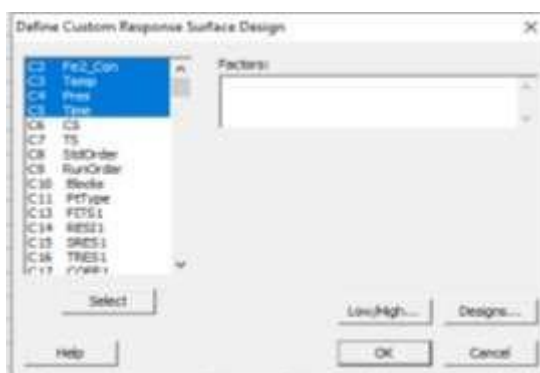
Figures 6. Selection of the four independent variables from the dialog box of Define Custom Response Surface Design.
