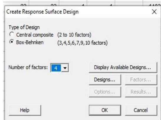
Figure 3. The dialog box used to select the Box-Behnken DOE and the number of independent variables (which is four) in each of the cement slurry systems.
