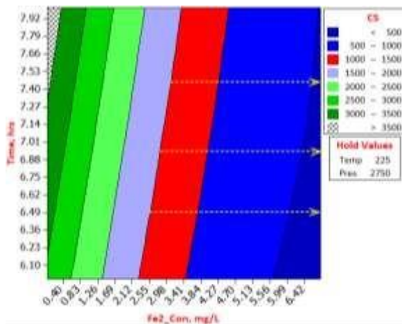
Figure 24. The Optimal Zone, Comfort Zone, and Adverse Zone of Compressive Strength in a Ferrous Cement Sheath System; which is depicted in the 3D Contour Plot of CS vs Time., and Fe2_Con., at Constant Temp. (225°F) and Pres. (2750psi).
