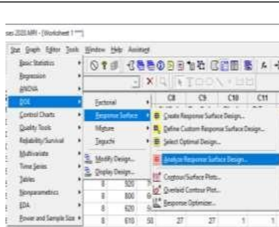
Figure 12. Selection of the analyse response design through STAT, DOE and RESPONSE SURFACE.
