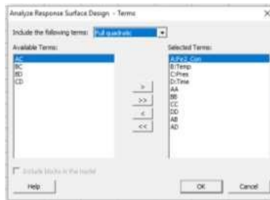
Figure 14. Selection of the optimal design probable model (Full Quadratic) from the Analyze Response Surface Design dialog box.
