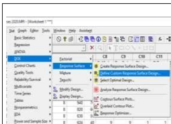
Figures 5. Definition of the Custom Response Surface Design through STAT, DOE and RESPONSE SURFACE, to select the available for four independent variables.
