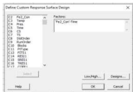
Figure 7. The four independent variables have been selected from the dialog box of Define Custom Response Surface Design.
