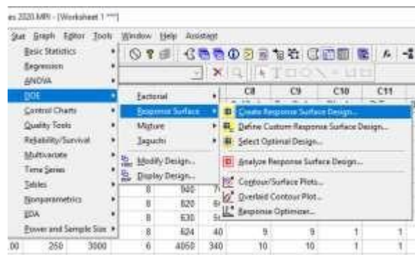
Figure 2. Creation of the Response Surface Design through STAT, DOE (Design of Experiment), and RESPONSE SURFACE.
