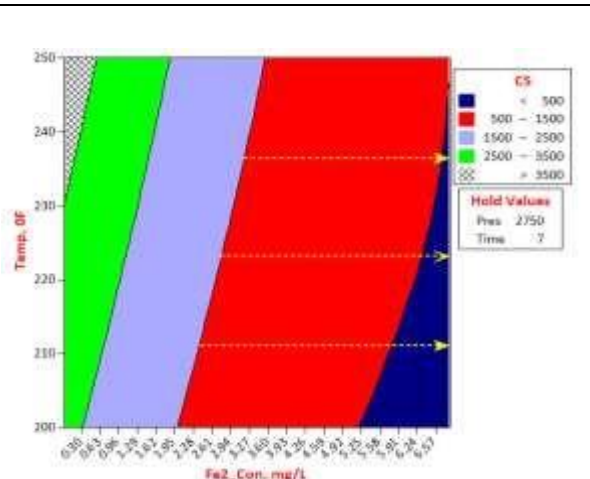
Figure 22. A 3D Contour Plot of CS vs Temp., and Fe2_Con., at Constant Pres. (2750psi) and Time (7hrs); Showing the Optimal Zone, Comfort Zone, and Adverse Zone of Compressive Strength in a Ferrous Cement Sheath System.
