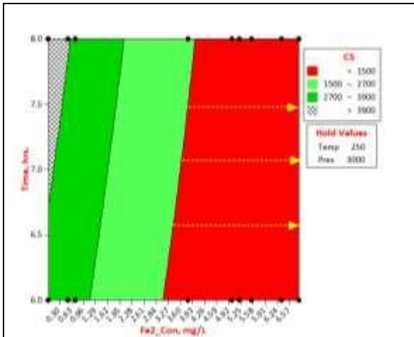
Figure 21. The Optimal Zone, Comfort Zone, and Adverse Zone of Compressive Strength in a Ferrous Cement Sheath System; which is depicted in the 3D Contour Plot of CS vs Time., and Fe2_Con., at Constant Temp. (250°F) and Pres. (3000psi).
