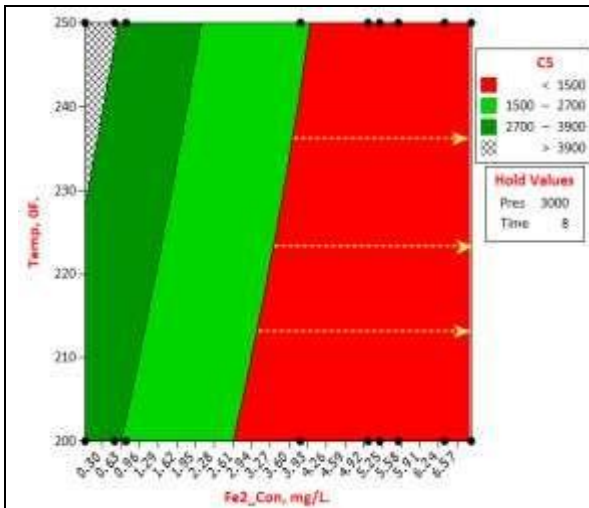
Figure 19. A 3D Contour Plot of CS vs Temp., and Fe2_Con., at Constant Pres. (3000psi) and Time (8hrs); Indicating the Optimal Zone, Comfort Zone, and Adverse Zone of Compressive Strength in a Ferrous Cement Sheath System.
