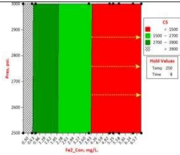
Figure 20. A 3D Contour Plot of CS vs Pres., and Fe2_Con., at Constant Temp. (250°F) and Time (8hrs); which Shows the Optimal Zone, Comfort Zone, and Adverse Zone of Compressive Strength in a Ferrous Cement Sheath System.
