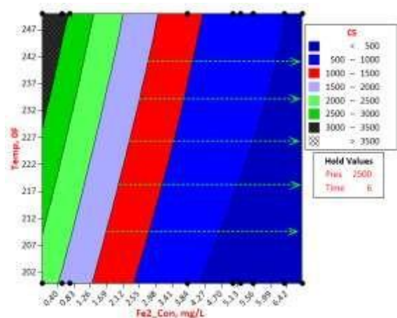
Figure 25. A 3D Contour Plot of CS vs Temp., and Fe2_Con., at Constant Pres. (2500psi) and Time (6hrs); which holds the Comfort Zone, and Adverse Zone of Compressive Strength in a Ferrous Cement Sheath System.
