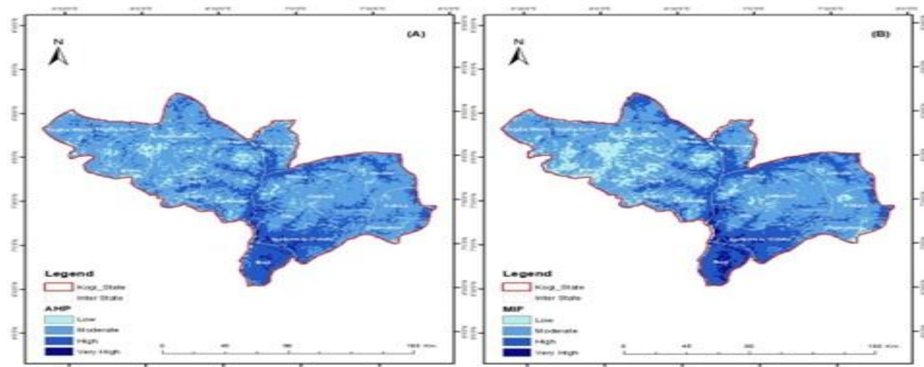
Figure 5: Flood vulnerability zones of Kogi state (A) AHP model map, (B) MIF model map.
